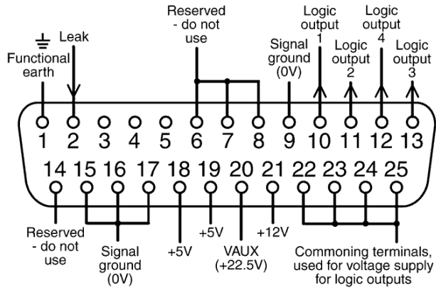
Upper D-connector
