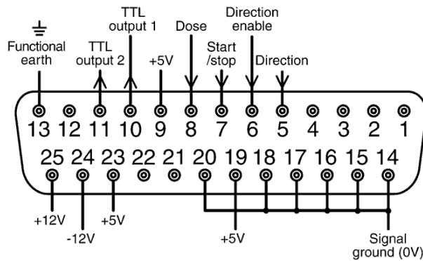
Lower D-connector
